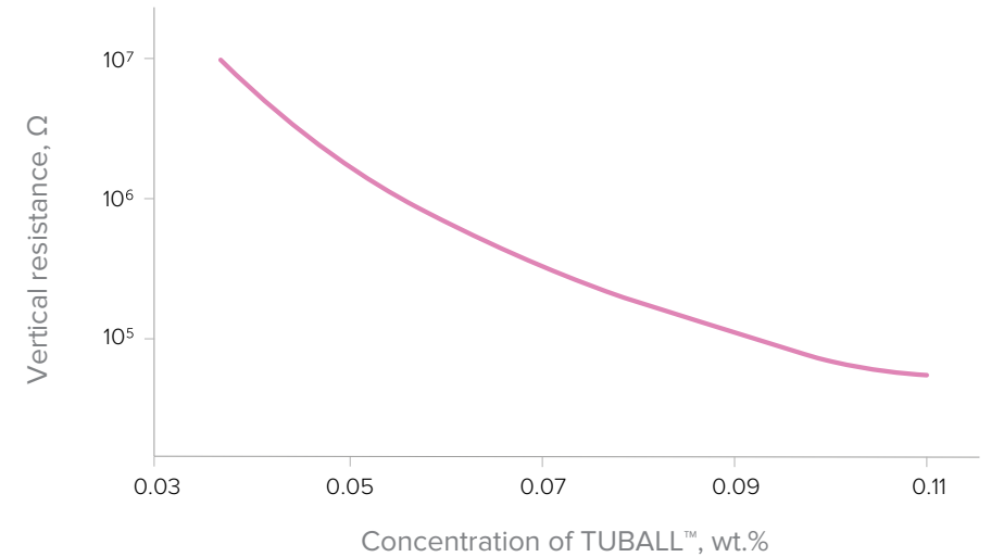
Measurement of electrical resistivity according to EN 16350:2014 carried out on teraohmmeter: TO-3 cable; electrode type - TE 50 for textile measurement (DIN 54345-1, DIN EN 1149-1 and DIN EN 1149-2)
