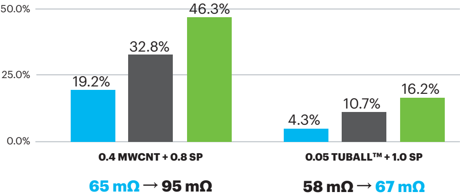
DCR increase during 45°C cell cycling
